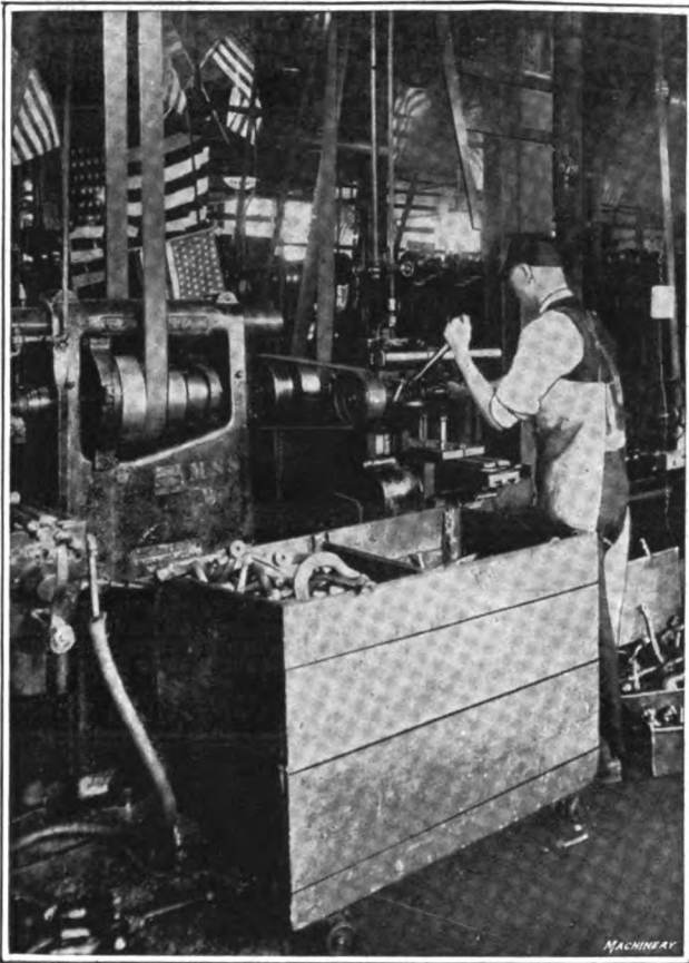
Fig. 5—Forgings, castings, etc., delivered to machines for a specified operation must be kept separate from those on which the operation has already been performed. One truck for blanks and one for machined work take up considerable space. A better method is to have one truck with a partition dividing the space into a compartment for blanks and a second compartment for finished work (Timken-Detroit Axle Co.)
